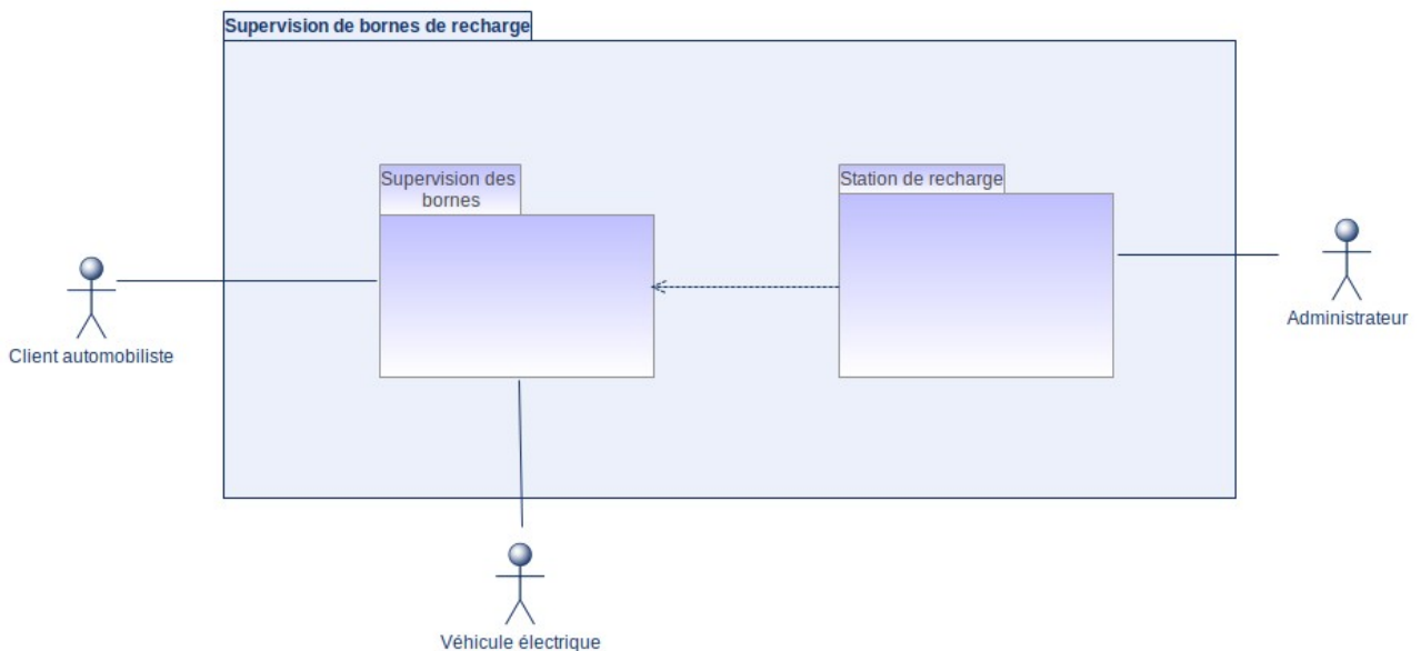
Figure 3: diagramme de packages – Supervision de bornes de recharge
